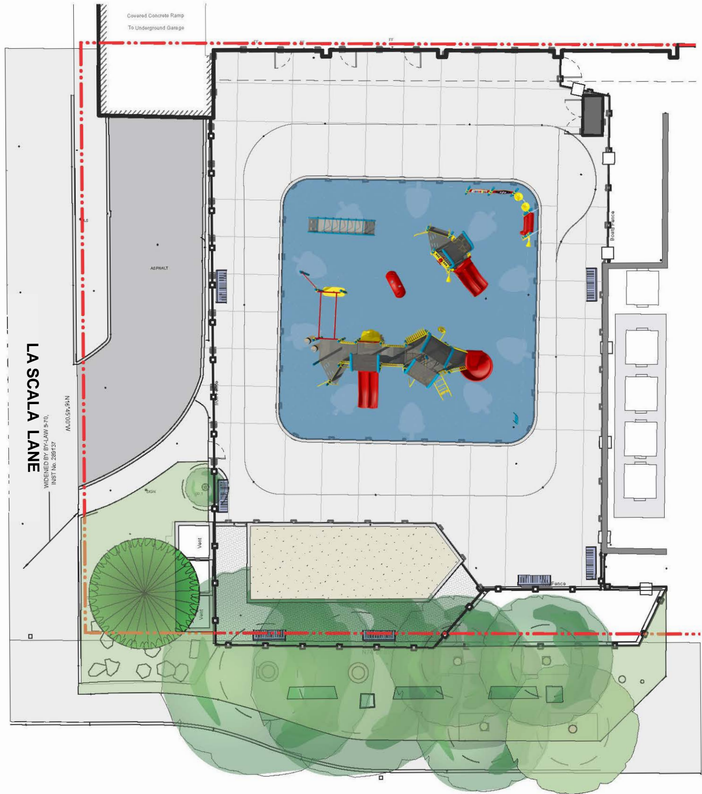
ST. MARY STREET PLAN
